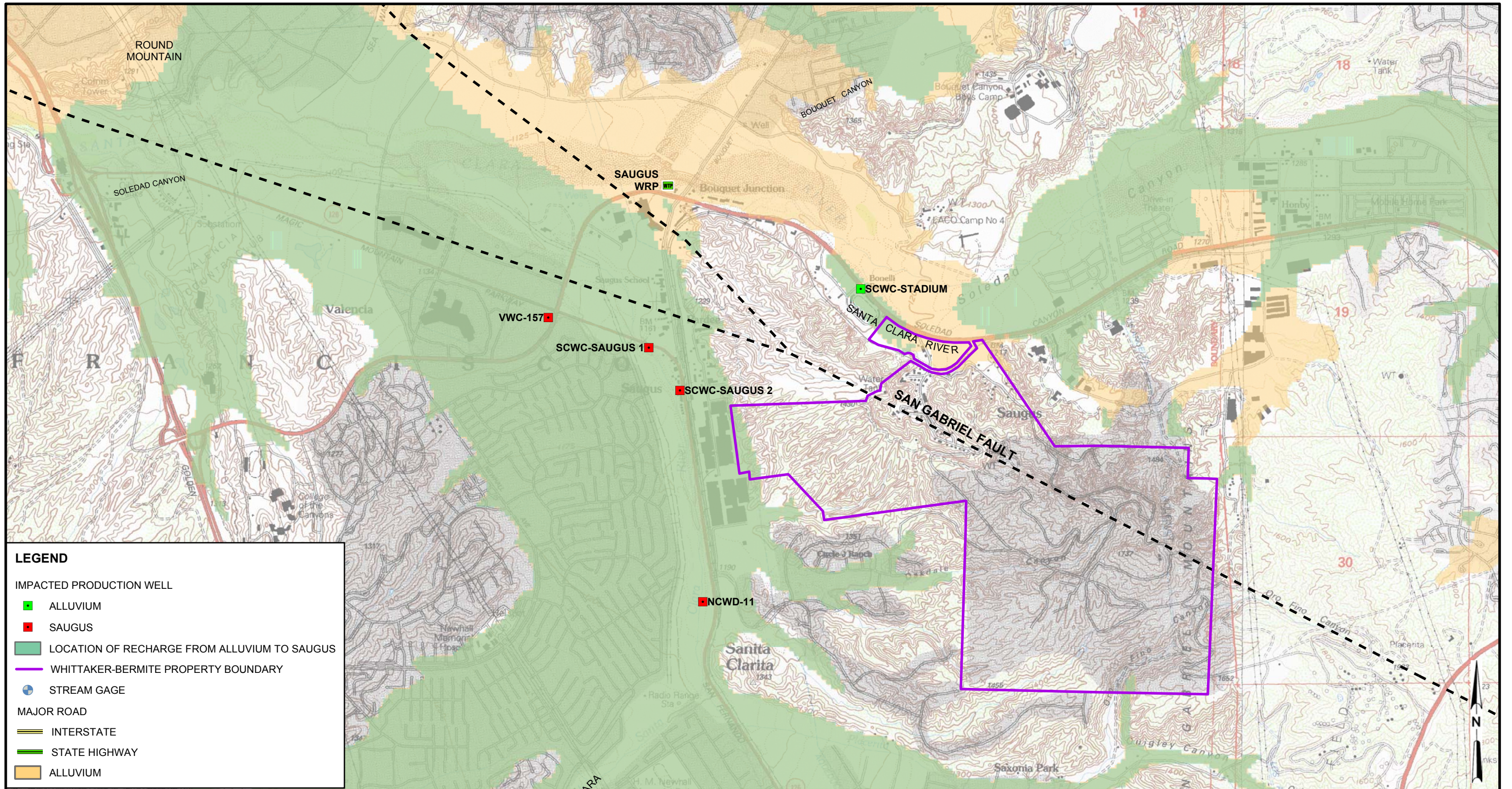
FIGURE 2-30 LOCATIONS OF SAUGUS FORMATION RECHARGE FROM THE ALLUVIAL AQUIFER IN THE VICINITY OF THE WHITTAKER-BERMITE PROPERTY ANALYSIS OF PERCHLORATE CONTAMINANT IN GROUNDWATER NEAR THE WHITTAKER-BERMITE PROPERTY SANTA CLARITA, CALIFORNIA
