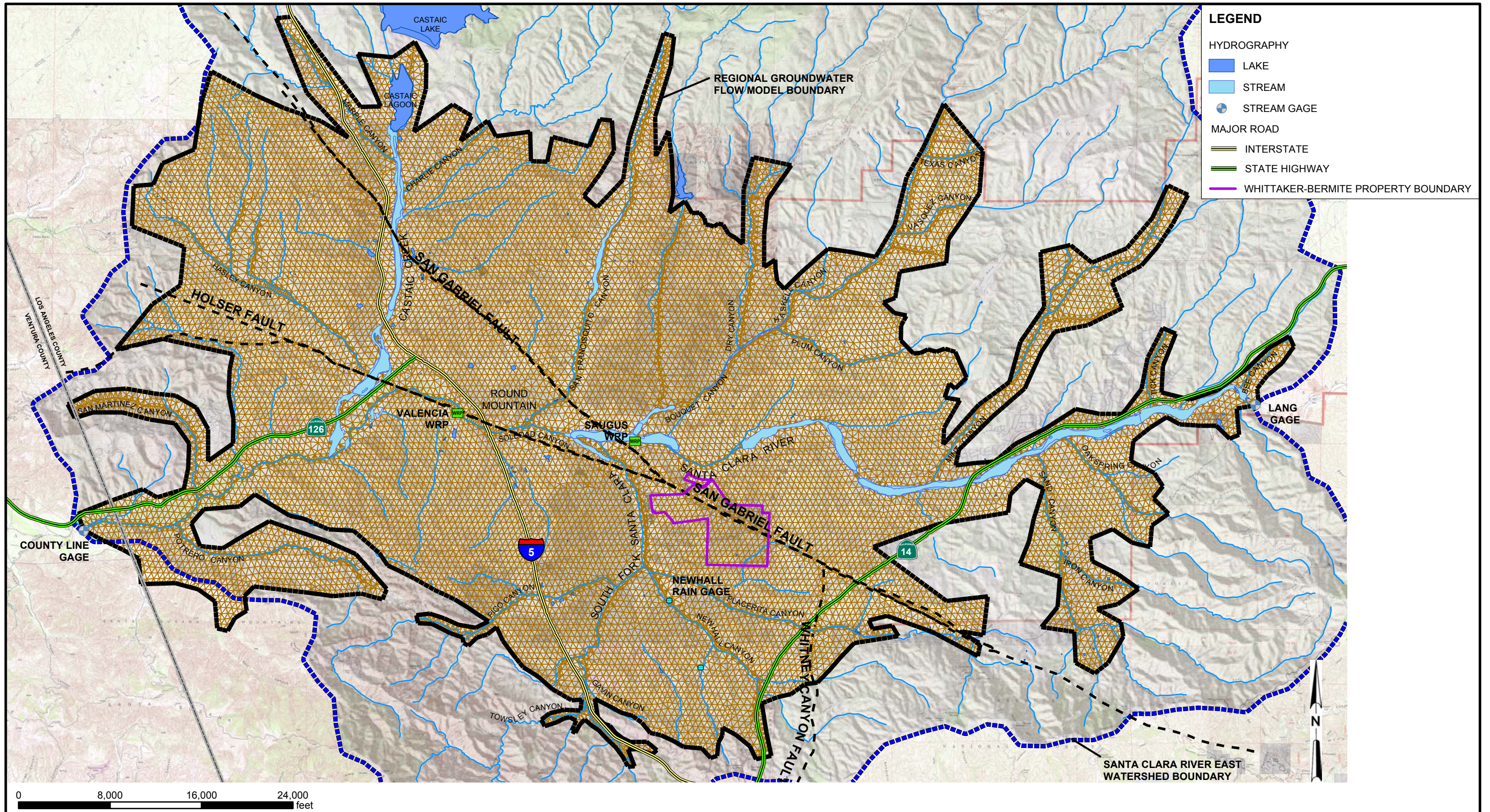
FIGURE 2-5 REGIONAL MODEL GRID ANALYSIS OF PERCHLORATE CONTAMINATION IN GROUNDWATER NEAR THE WHITTAKER-BERMITE PROPERTY SANTA CLARITA, CALIFORNIA
