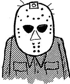
JASON
