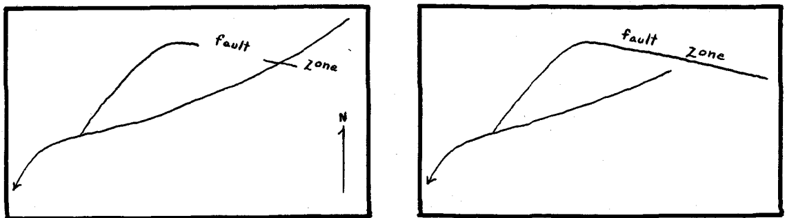
Figure 12 - Diagram of autopiratic stream capture along the San Gabriel fault zone.
