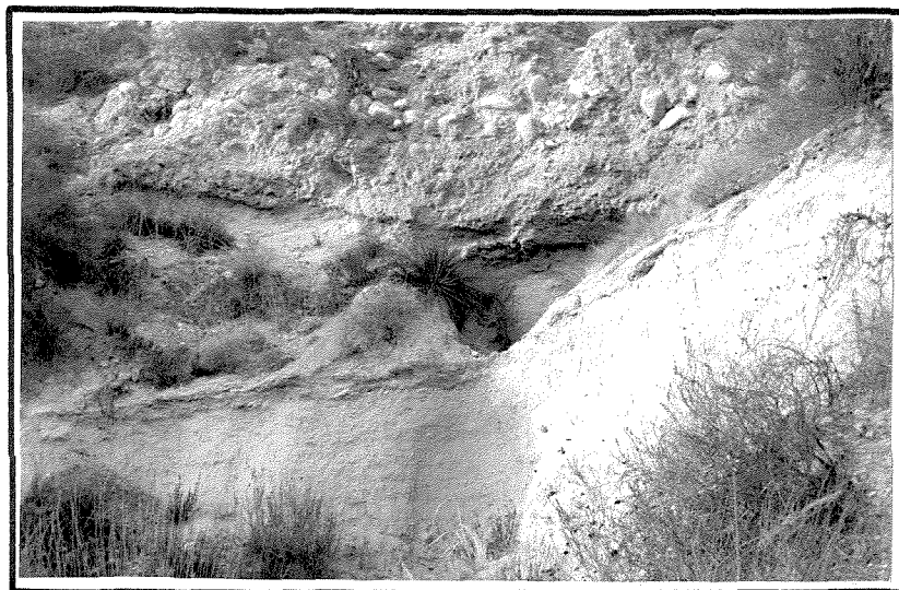
Figure 4 - Angular unconformity between Pico strata and overlying Saugus beds at the point Sec. 31 (30-12) in Placerita Canyon.
